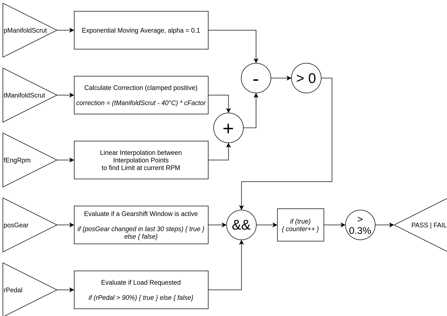
Figure 1: Boost Monitoring Method Block Diagram
